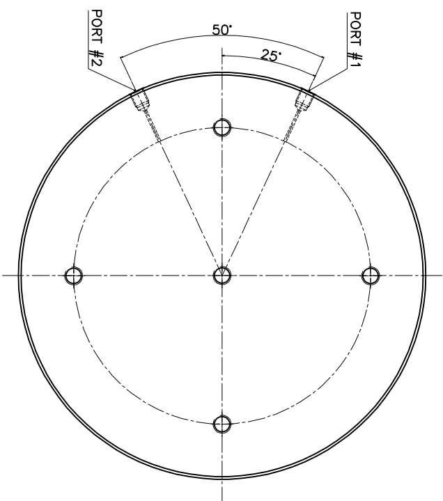
VIEW "A"
