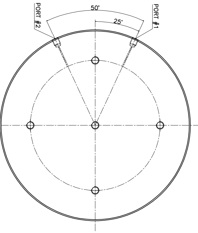
VIEW "A"
