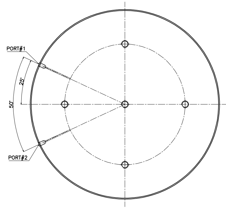
VIEW "A"
