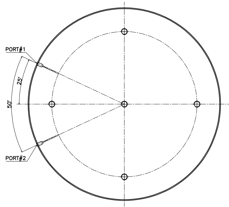
VIEW "A"
